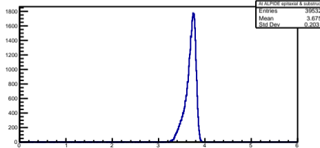
Lossed Energy in ALPIDE epitaxial + substruct at Alpha (d = 24mm)
