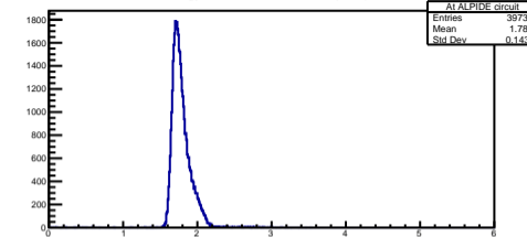
Lossed Energy in ALPIDE circuit at Alpha (d = 24mm)
